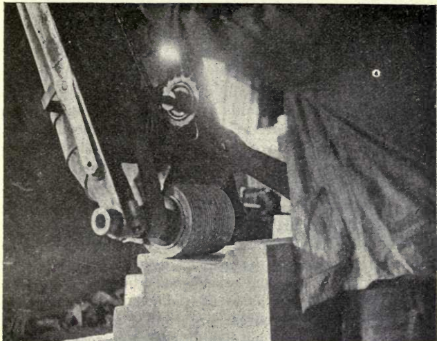
FIG. 80—MACHINE FOR FINISHING CONCRETE IN PARALLEL CUTS OF FROM \frac{1}{8} " TO \frac{1}{4} " WIDE
